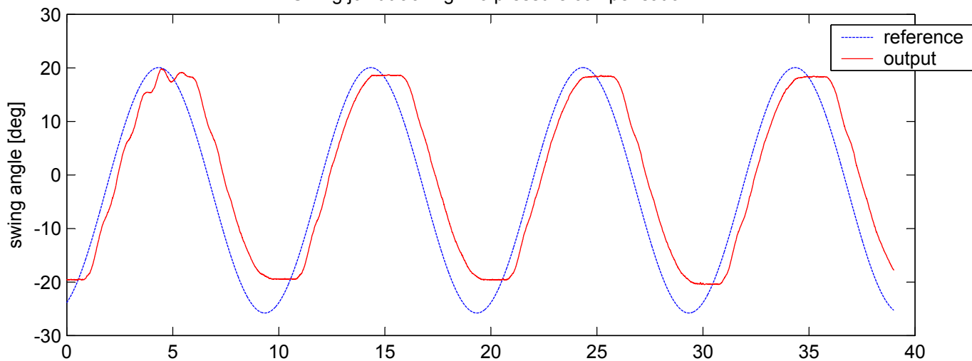
Swing joint tracking w/o pressure compensation
