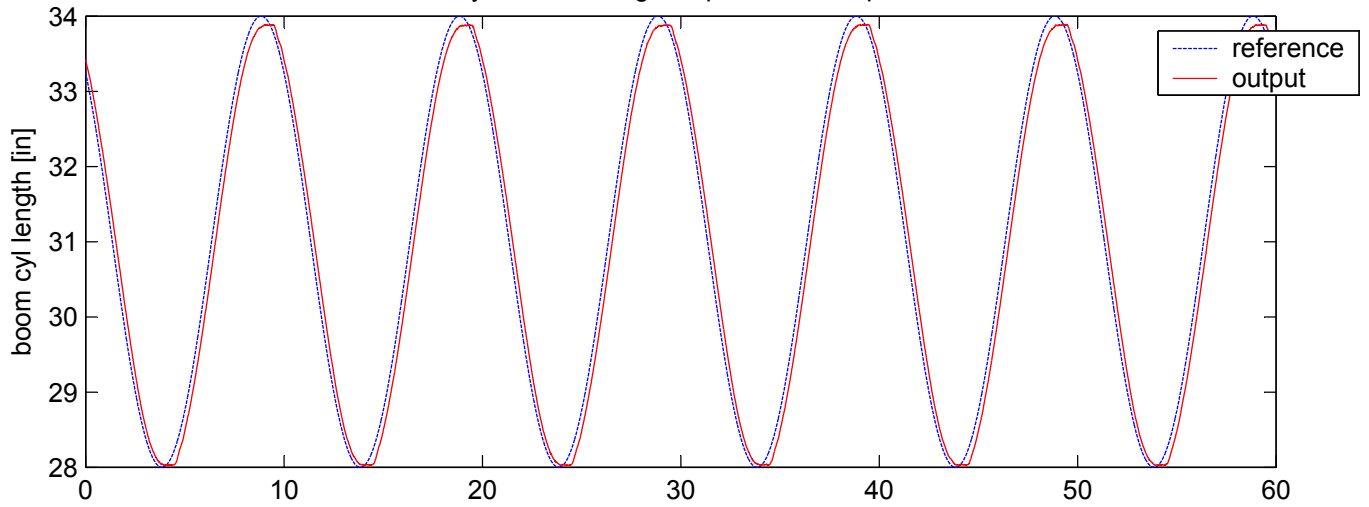
Boom cylinder tracking w/o pressure compensation
